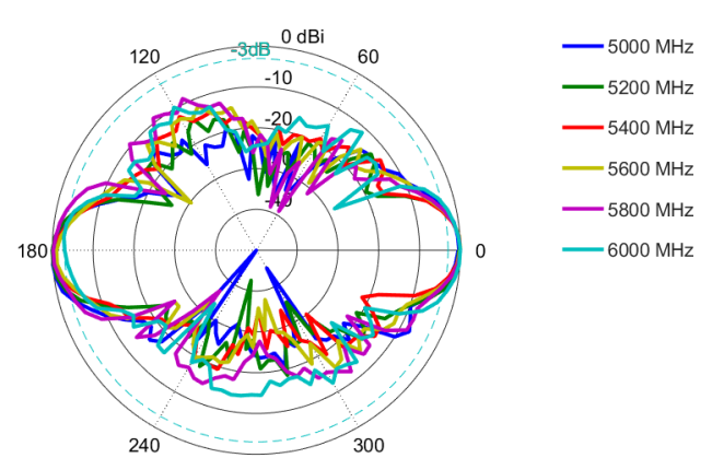
Elevation Port 1 & 3: 2400 – 2500MHz | Elevation Port 2 & 4: 5000 – 6000 MHz
