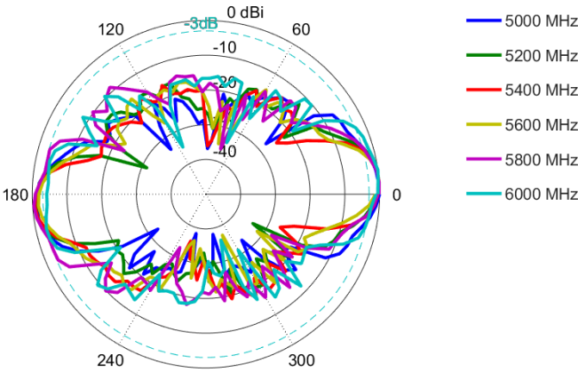
Azimuth Port 1 & 3: 2400 – 2500MHz | Azimuth Port 2 & 4: 5000 – 6000 MHz
