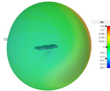
3D Pattern Element 1 (850MHz)
