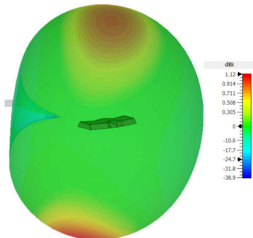
3D Pattern Element 2 (1800MHz)
