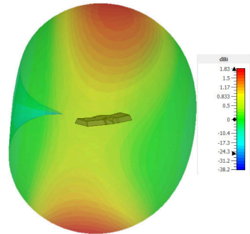
3D Pattern Element 2 (850MHz)
