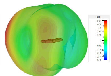
3D Pattern Element 2 (3500MHz)
