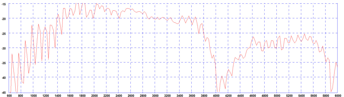
Typical Isolation - WiFi Elements 4-5*
