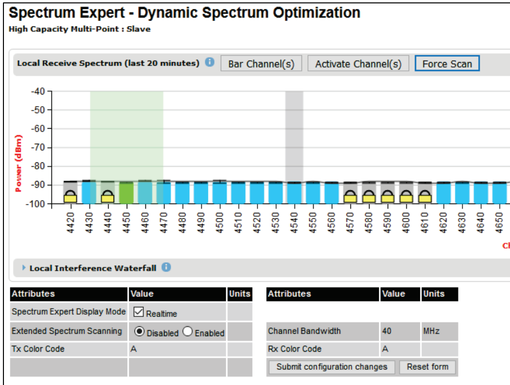
Figure 205 Spectrum Expert page with Slave Scan
