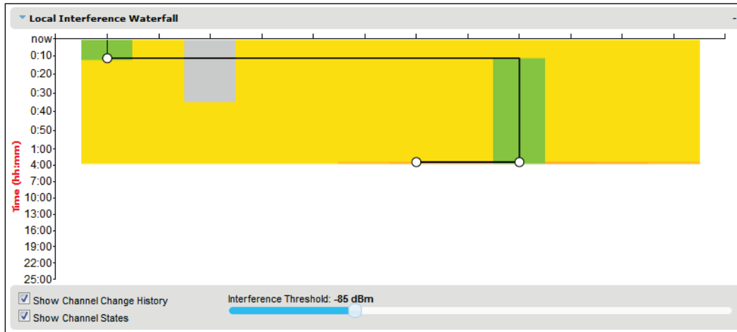
Figure 218 Spectrum Expert page, Interference Waterfall plot with channel states
