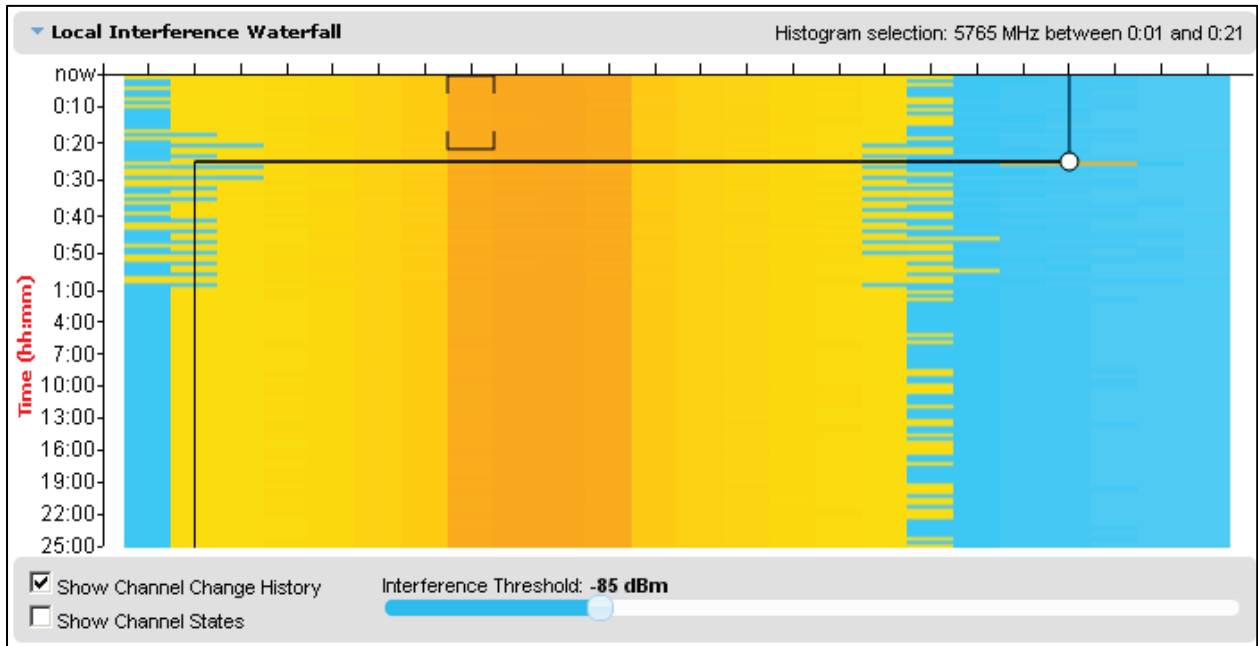
Figure 216 Spectrum Expert, Interference Waterfall plot
