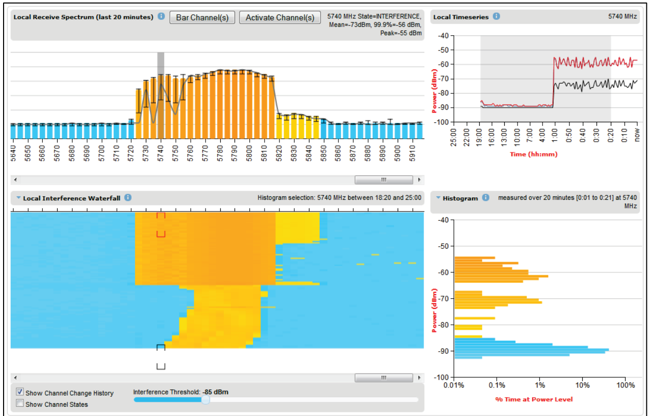
Figure 221 Spectrum Expert, example 2
