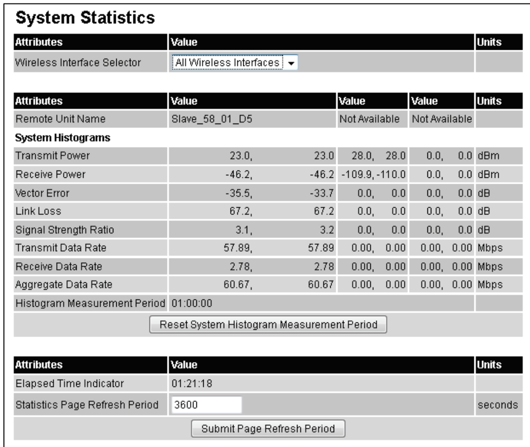
Figure 225 System Histograms section of the System Statistics page (HCMP Topology, Wireless Interface Selector set to “All Wireless Interfaces”)
