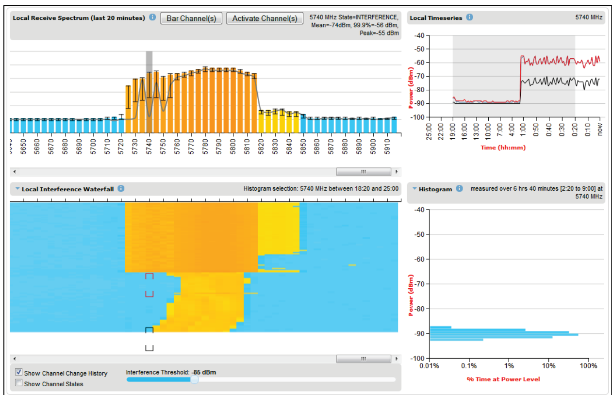
Figure 220 Spectrum Expert, example 1
