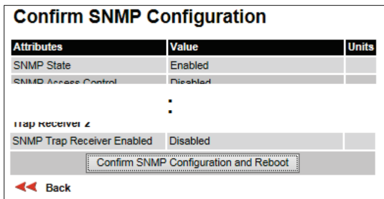
Figure 162 Confirm SNMP Configuration page (for SNMPv3) (top and bottom of page shown)
