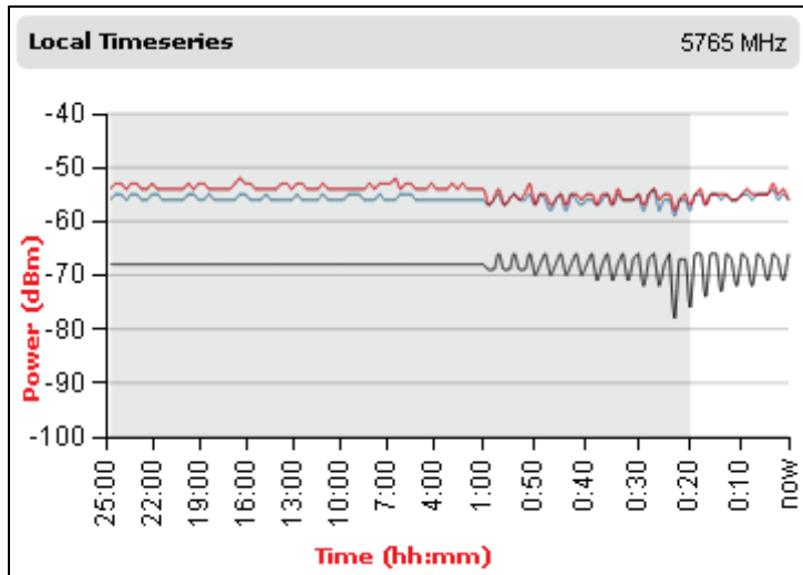
Figure 215 Spectrum Expert, Timeseries plot
