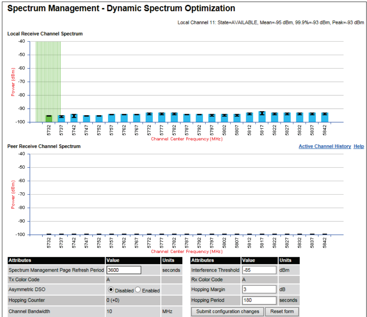
Figure 206 Spectrum Management page (Master unit)
