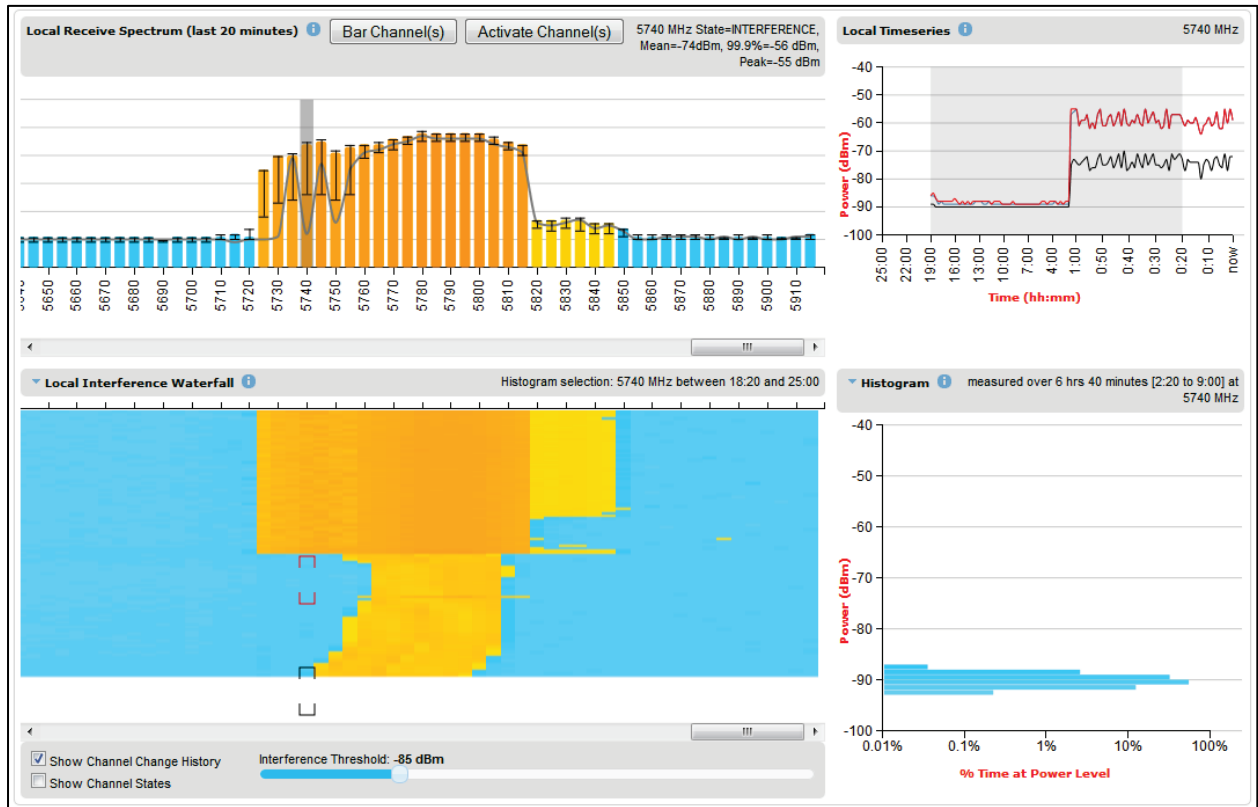
Figure 214 Selecting a channel on the Receive Spectrum
