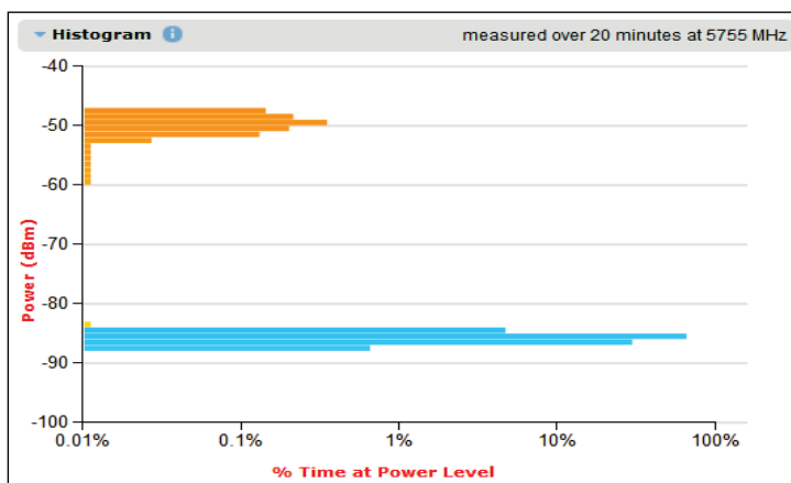
Figure 219 Spectrum Expert page, histogram plot
