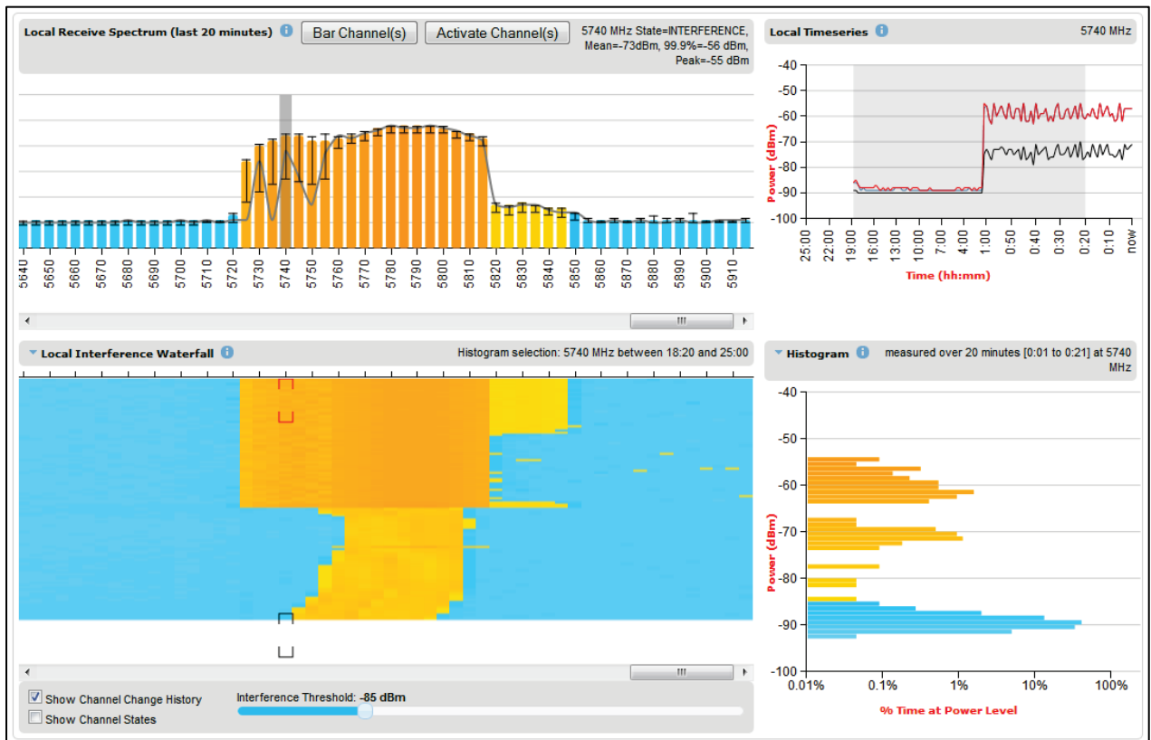
Figure 204 Spectrum Expert page showing the Receive Spectrum, Timeseries, Interference Waterfall and Histogram for the Local unit
