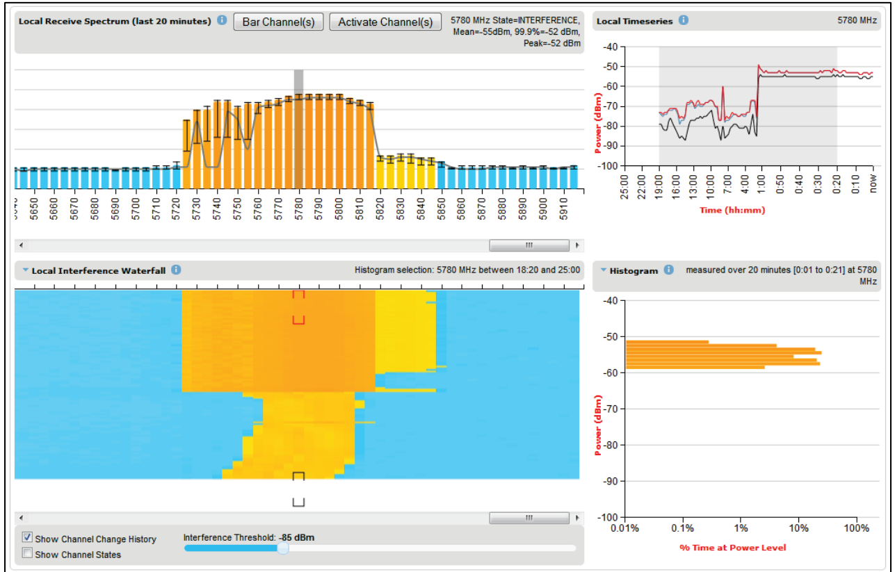
Figure 222 Spectrum Expert, example 3
