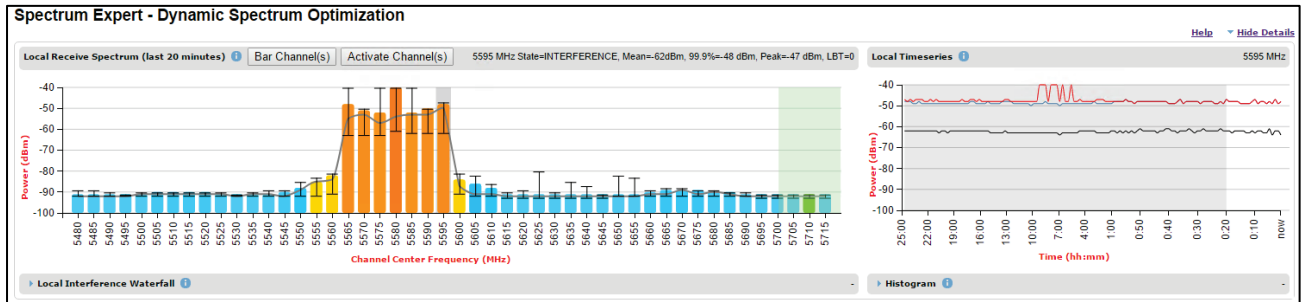
Figure 202 Spectrum Expert page with Receive Spectrum and Timeseries for the Local unit
