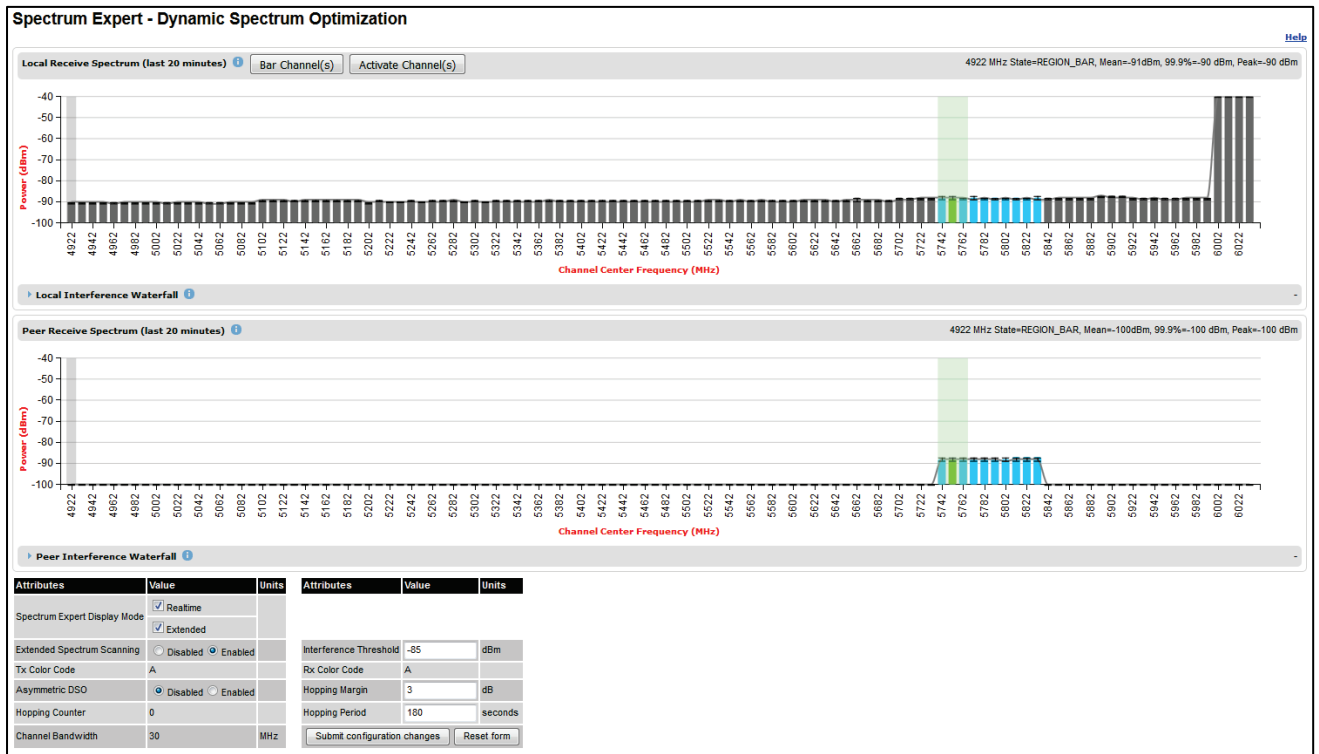
Figure 201 Spectrum Expert page - Extended Display mode
