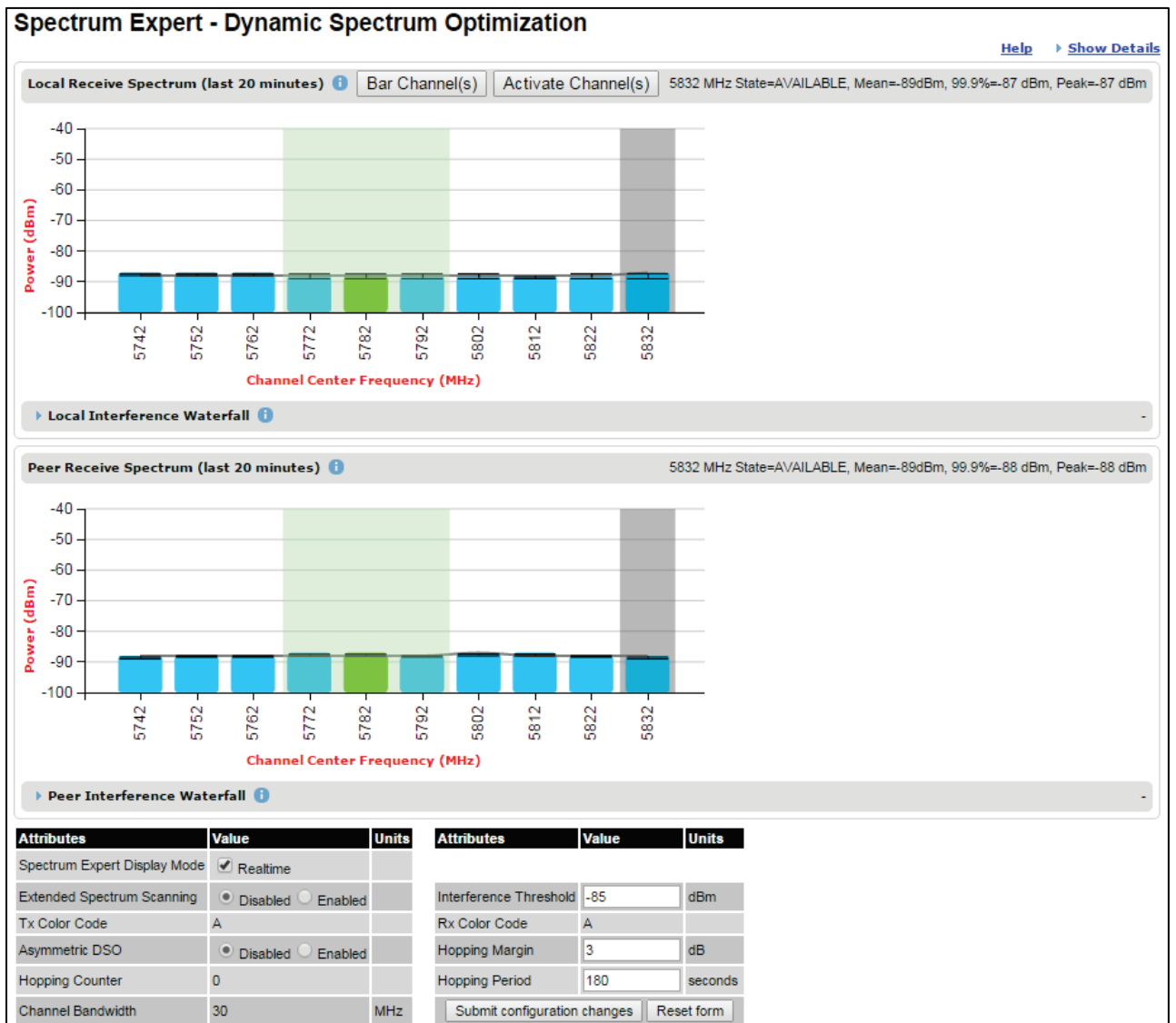
Figure 200 Spectrum Expert page - Standard Display mode
