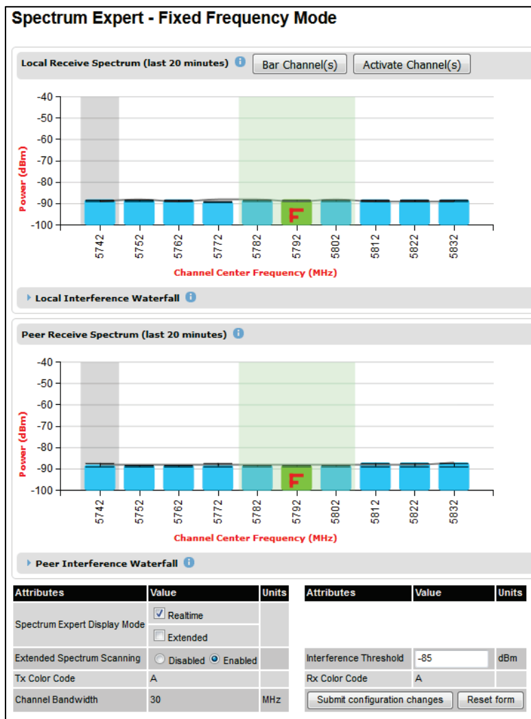
Figure 207 Spectrum Expert page for Fixed Frequency - Standard display mode
