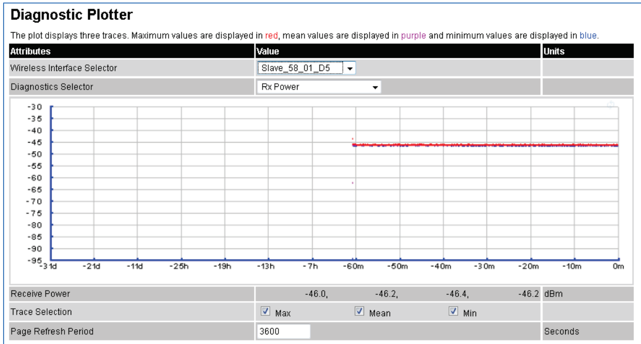
Figure 239 Diagnostic Plotter page (HCMP topology)
