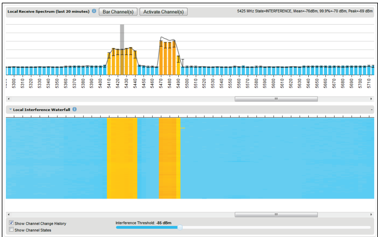
Figure 203 Spectrum Expert page showing the Receive Spectrum and Interference Waterfall for the Local unit
