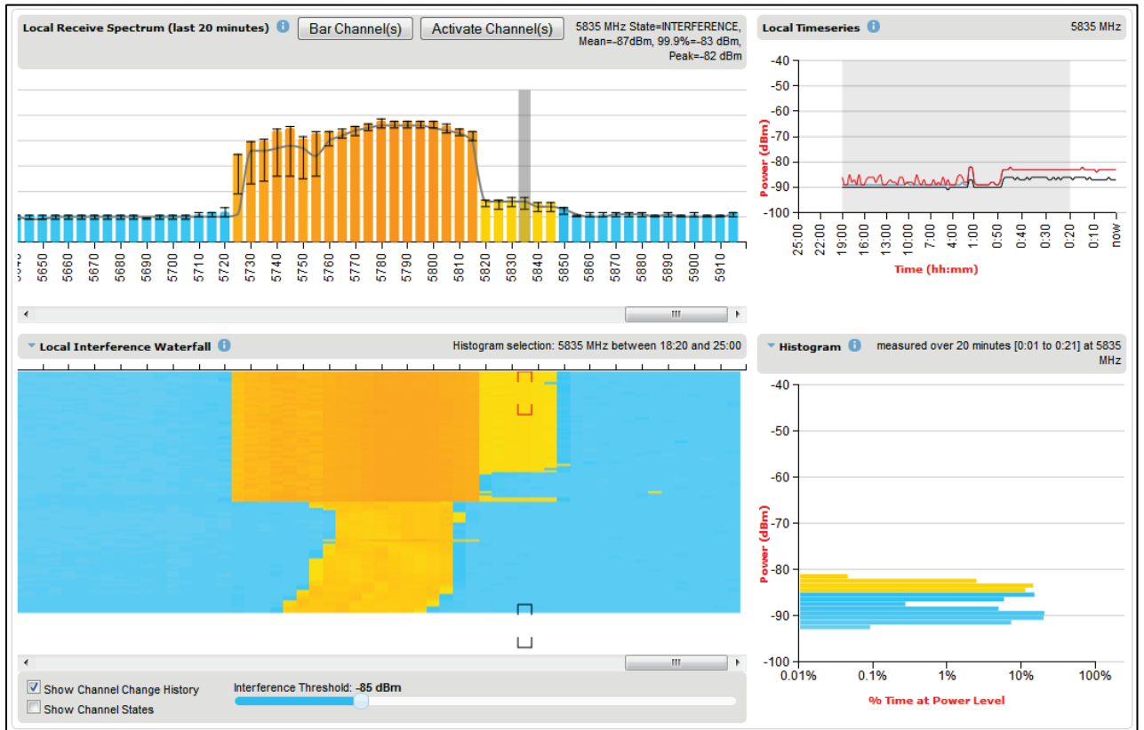
Figure 223 Spectrum Expert, example 4
