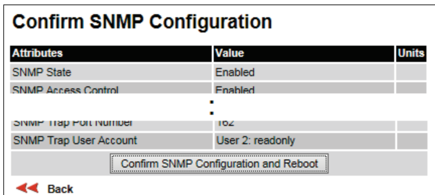
Figure 165 Confirm SNMP Configuration page (for SNMPv1/2c) (top and bottom of page shown)
