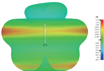
3D Plot Bottom Element (1800MHz)
