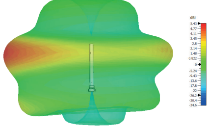
3D Plot Bottom Element (1800MHz)
