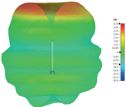
3D Plot Top Element (3600MHz)
