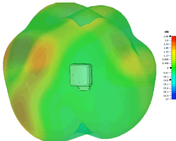
3D Gain Plot (2600MHz)
